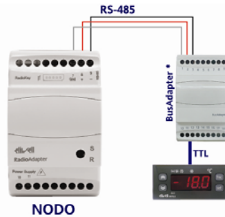
RadioAdapter/S + BusAdapter + instrument without RS-485
